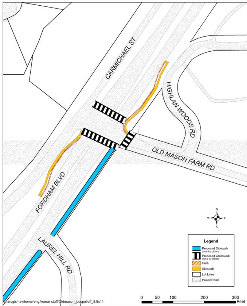
Proposed Bus Pulloffs for Fordham Blvd. at Old Mason Farm Rd and Christopher Rd
