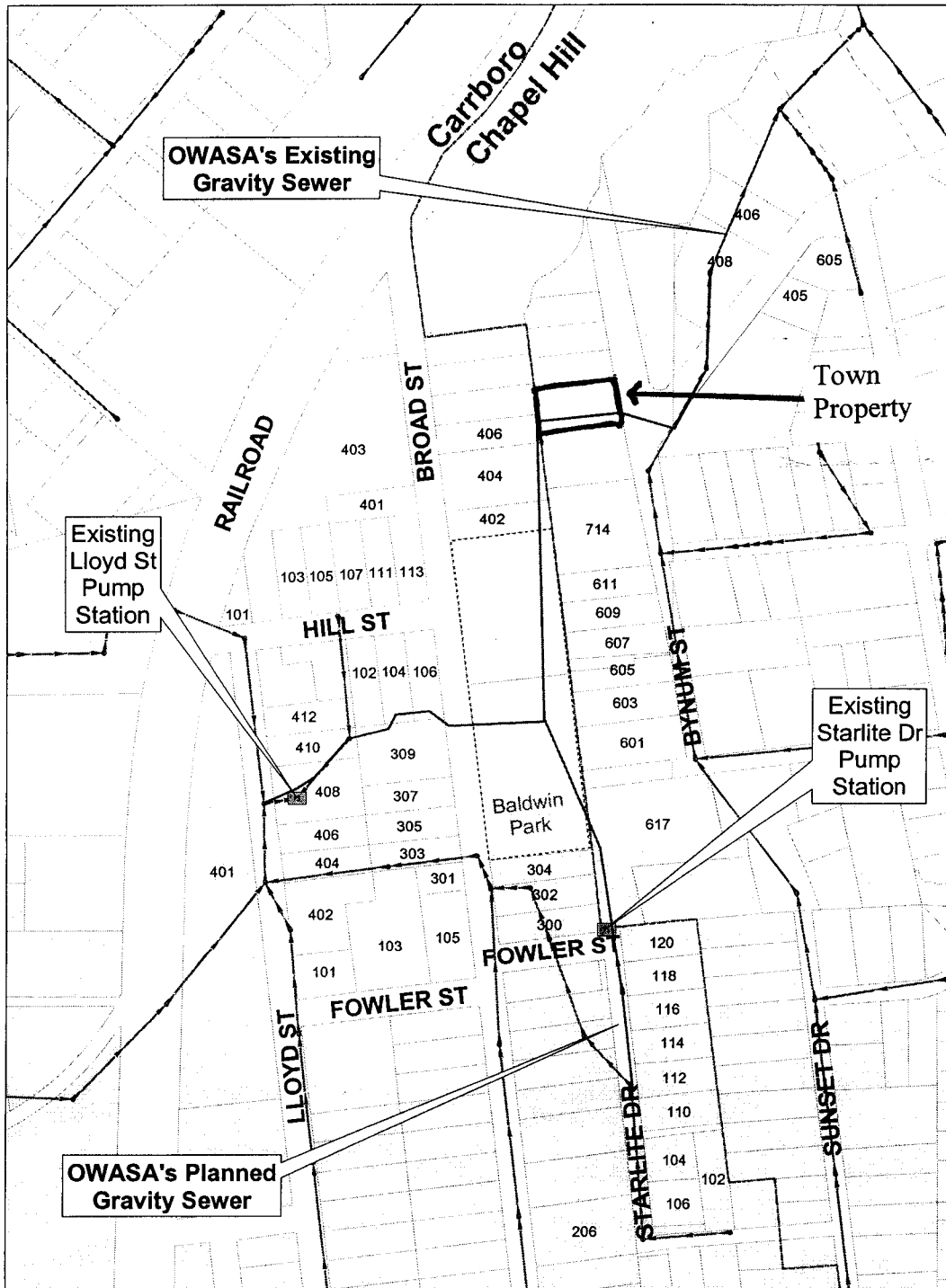
Approximate Location of New Sewer Following Closing of Lloyd St. & Starlite Dr. Pump Stations
