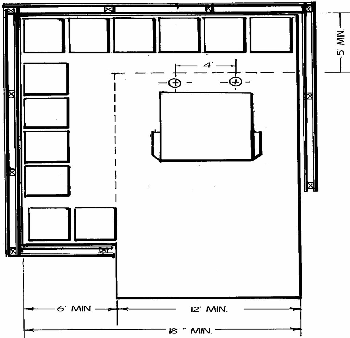
TYPICAL SINGLE WITH ROLLOUT CARTS
