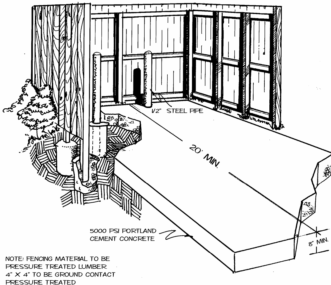
STANDARD DUMPSTER PAD WITH FENCING
