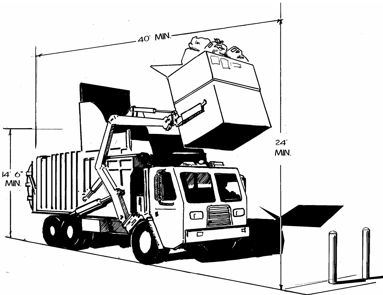
REFUSE TRUCK OVERHEAD CLEARANCE
