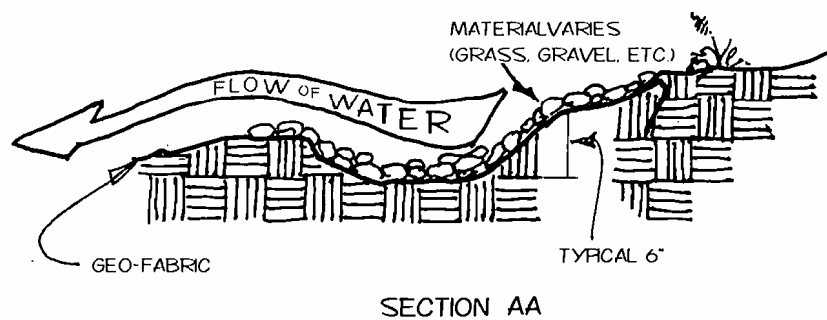
TYPICAL LEVEL SPREADER
