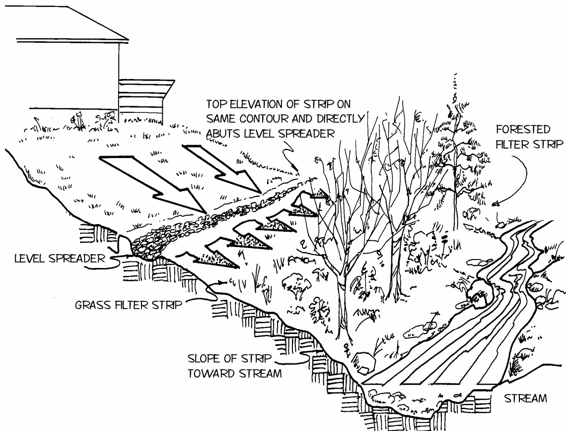
Figure 2.1: Filter Strip
