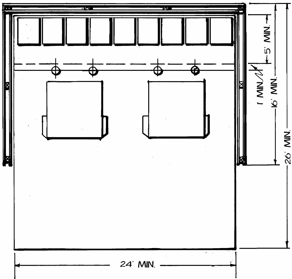
TYPICAL DOUBLE WITH ROLLOUT CARTS
