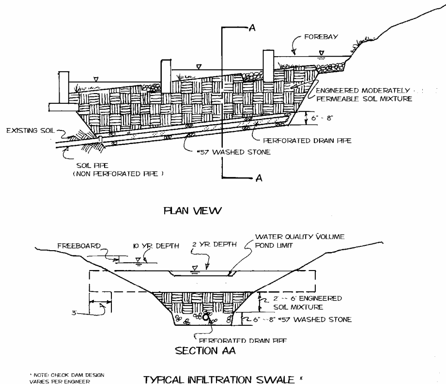
Figure 2-2.1 – A Typical Infiltration Swale
