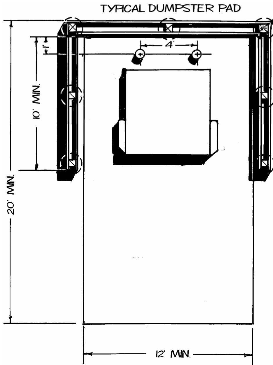
Diagram 1. Standard Typical single dumpster pad with screening fence erected adjacent to pad
