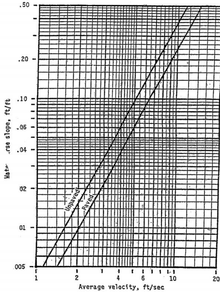
FIGURE 2-B-1 AVERAGE VELOCITIES FOR ESTIMATING TRAVEL TIME FOR SHALLOW CONCENTRATED FLOW
