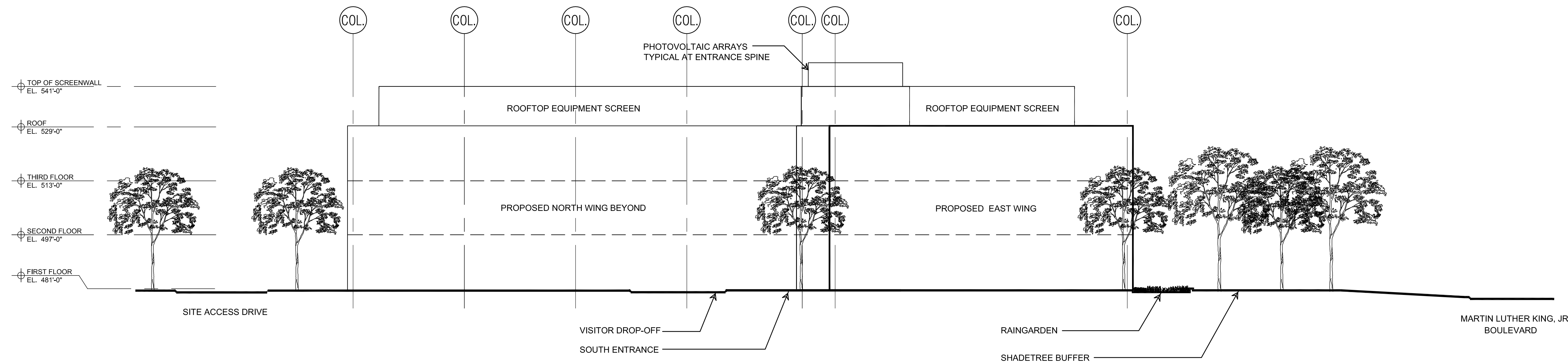
SOUTH ELEVATION
