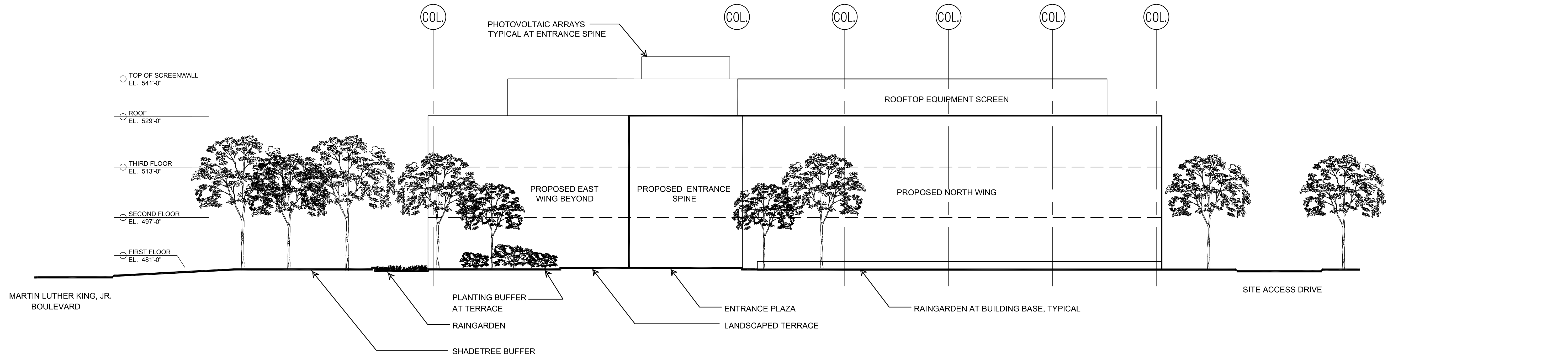
NORTH ELEVATION
