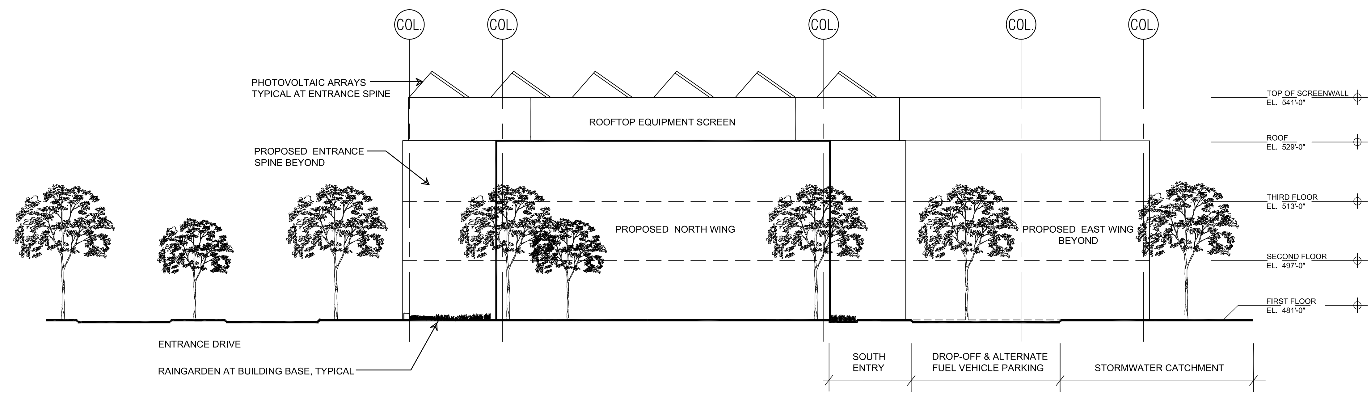
WEST ELEVATION
