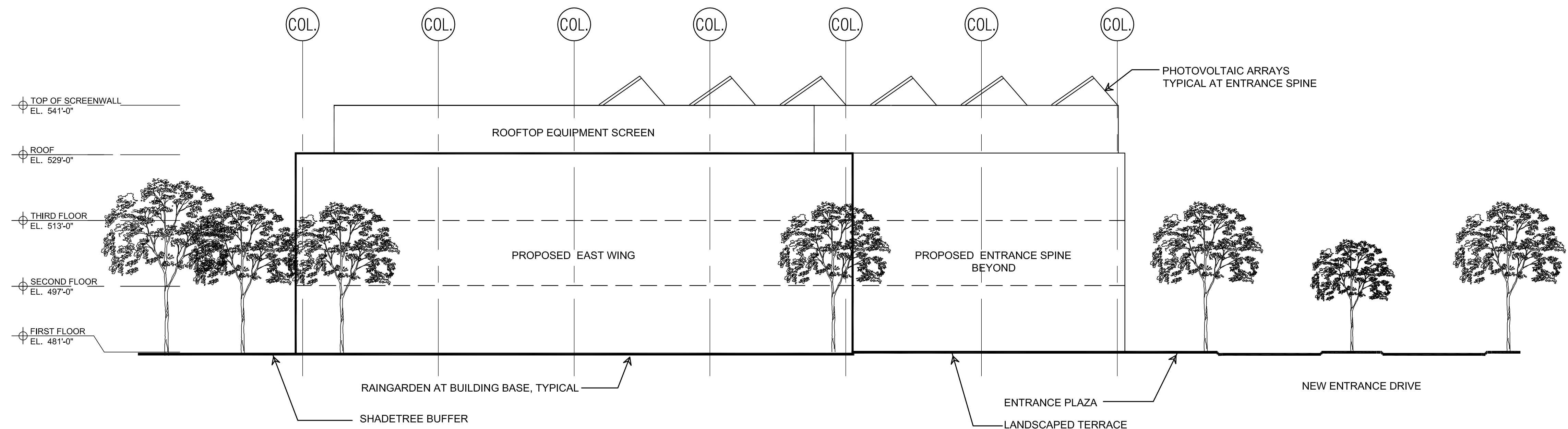
EAST ELEVATION
