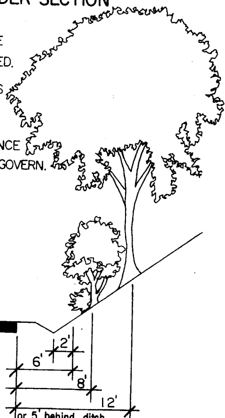
OUTSIDE or CUT SLOPE SECTION
