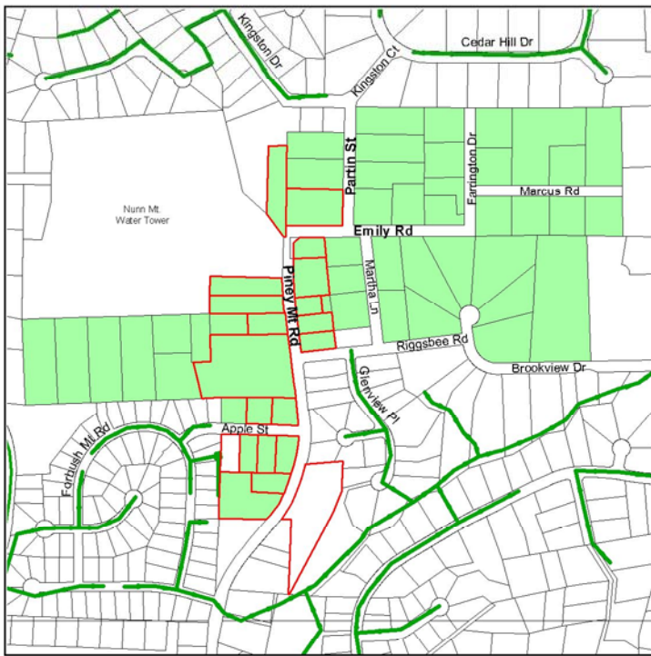
Piney Mtn. Rd / Emily Rd / Partin St Area with Existing Sewer Lines and Unsewered Lots
